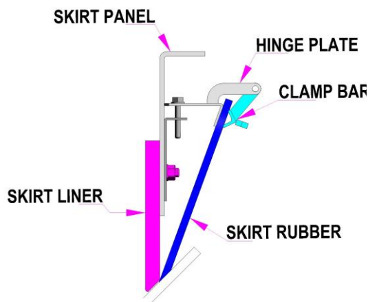
a. with clamp bar
