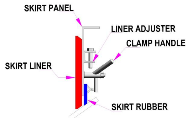
b. with clamp handle
