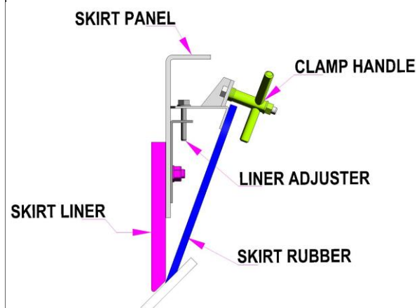
b. with clamp handle
