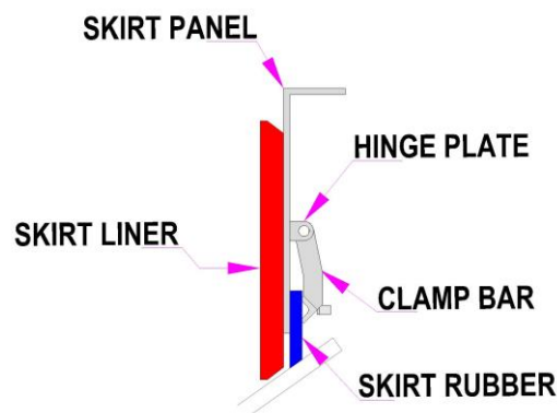
a. with clamp bar
